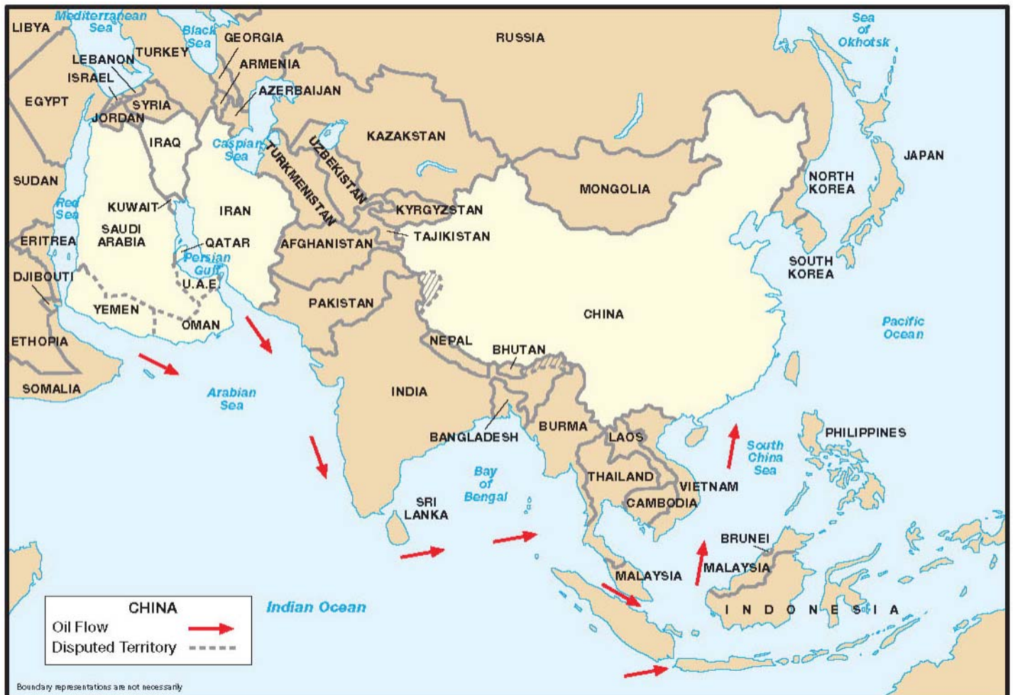
Figure 1. China's Critical Sea Lanes. China is heavily dependent upon critical sea lanes for its energy imports. Some 80% of China's crude oil imports transit the Straits of Malacca.
