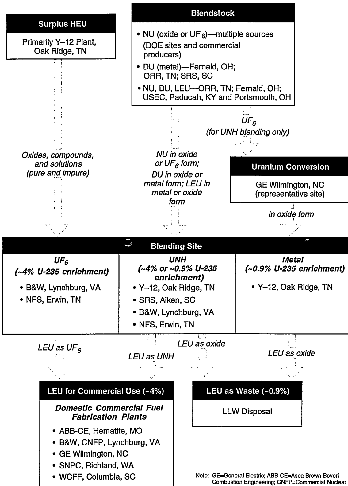
Figure S-3. Material Flow Diagram for Surplus Highly Enriched Uranium Disposition.
